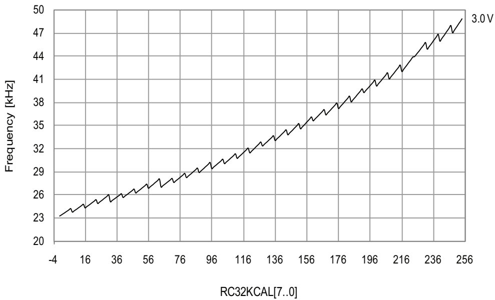
Figure 33-56. 32.768kHz Internal Oscillator Frequency vs. Calibration Value
