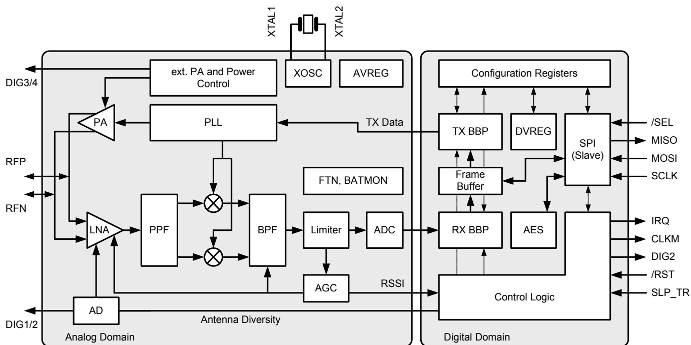
Figure 4-1. AT86RF231 Block Diagram
