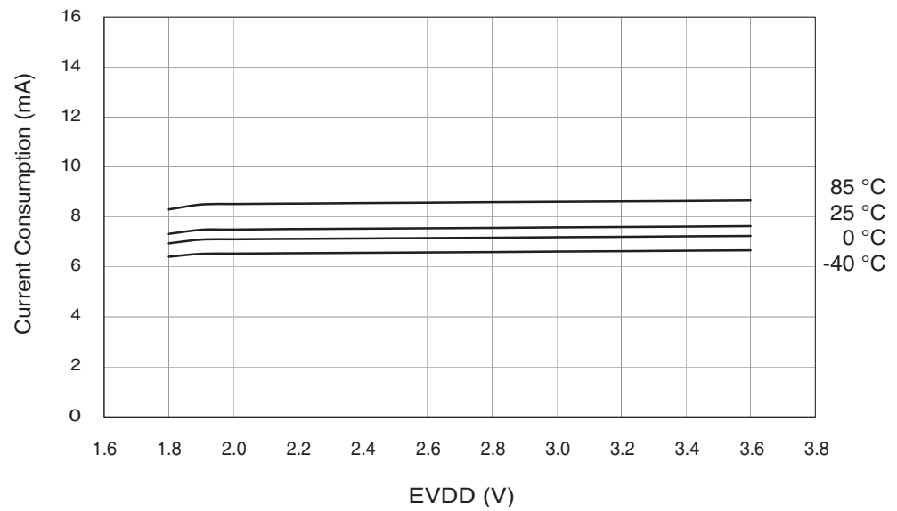
Figure 13-7. Current Consumption in TX_BUSY State - Minimum Output Power
