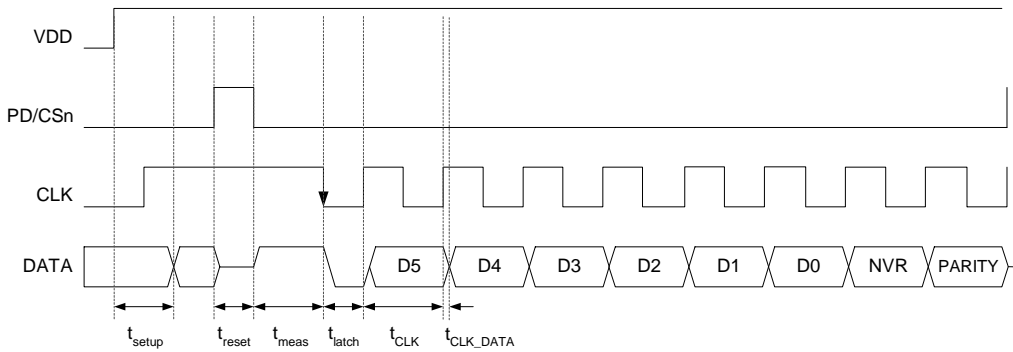
Figure 4 Timing diagram in Single Read Out mode
