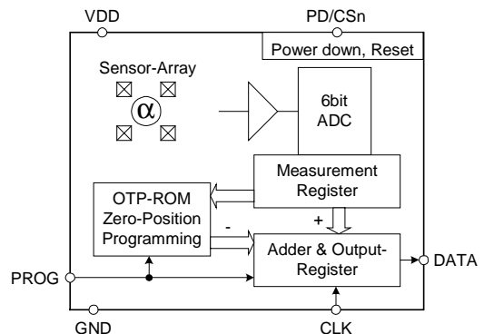
Figure 2 Block diagram
