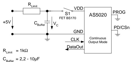
Figure 8 Schematics for basic low power application
