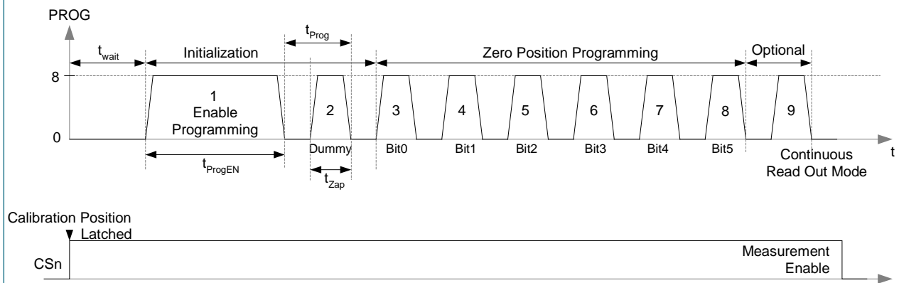
Figure 6 Programming sequence
